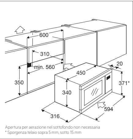
MW17E10M / MW17EG10M incasso in pensile
