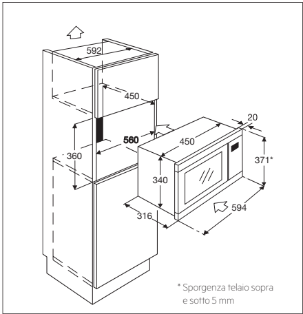
MW17E10M / MW17EG10M incasso in armadio a colonna
